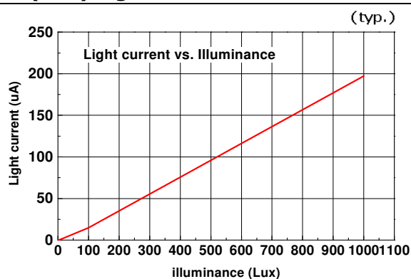
Fig.6 (LED) Light Current vs. Illuminance
