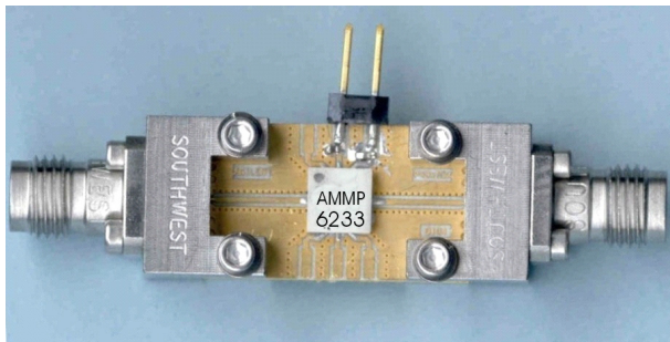
Figure 14. Evaluation / Test Board (Available to qualified customer requests)
