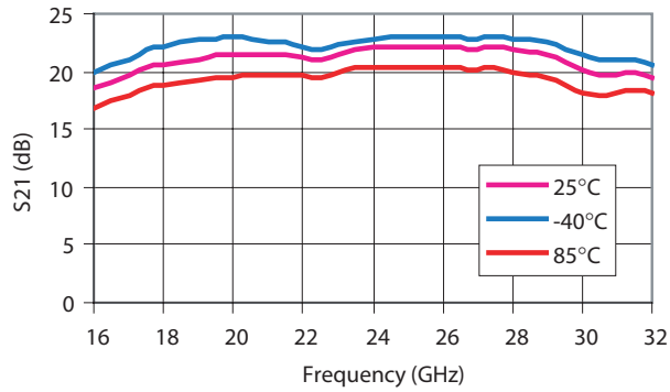
Figure 9. Gain over Temperature
