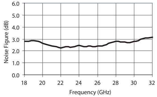
Figure 2. Noise Figure
