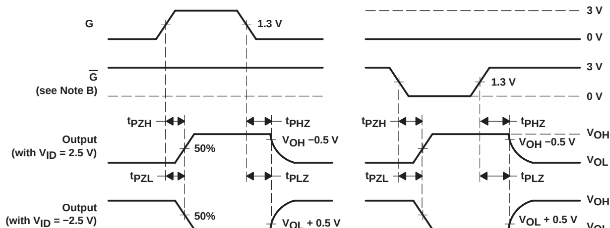
VOLTAGE WAVEFORMS
