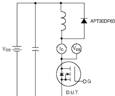
Figure 20, Inductive Switching Test Circuit
