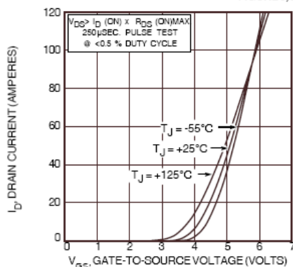
FIGURE 4, TRANSFER CHARACTERISTICS
