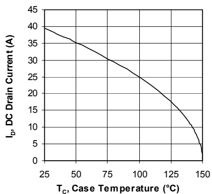
Figure 6, DC Drain Current vs Case Temperature
