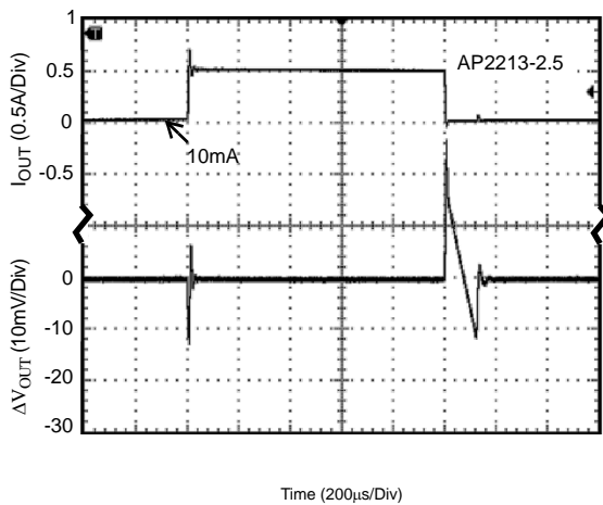
Figure 12. Load Transient
