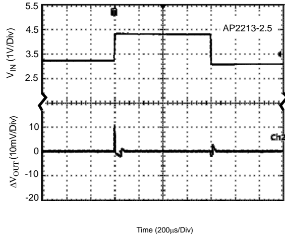
Figure 13. Line Transient
