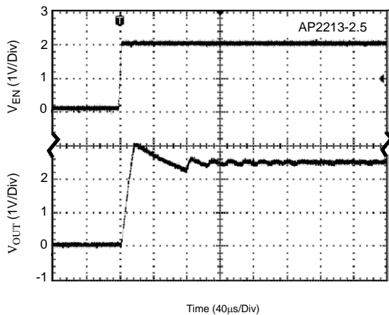
Figure 14. V_{EN} vs. V_{OUT}
