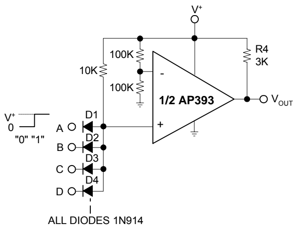
AND Gate
