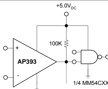
Driving CMOS
