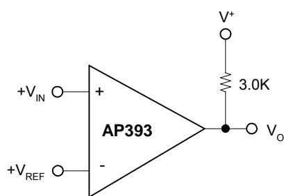
Basic Comparator
