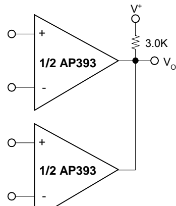
ORing the Outputs
