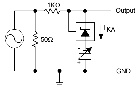
Test Circuit for Reference Impedance
