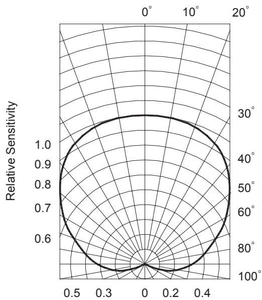
Figure 7. Sensitivity Diagram
