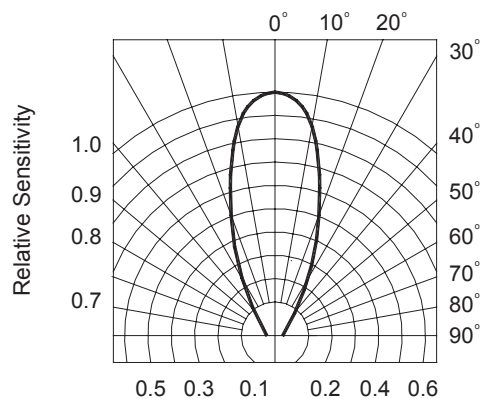
FIGURE 5. SENSITIVITY DIAGRAM
