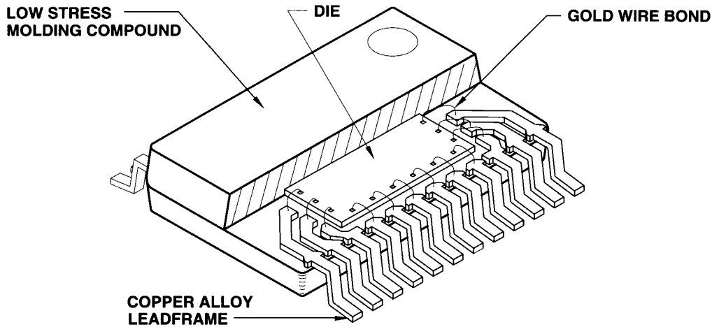
Figure 23: SSOP Package
