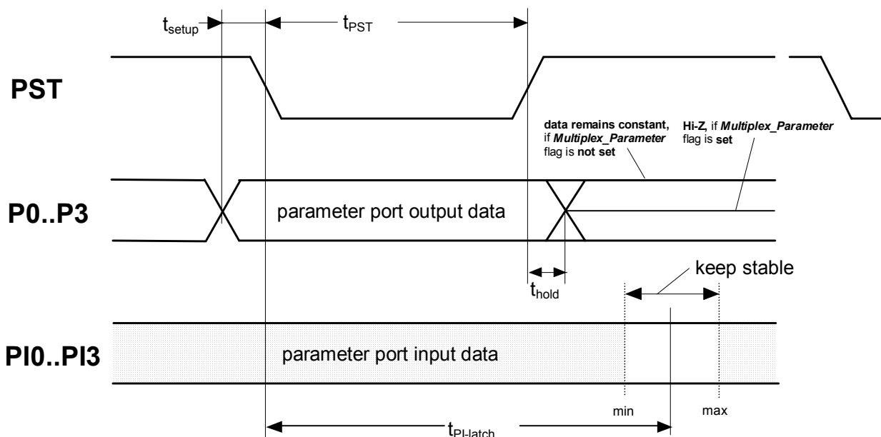
Figure 9: Timing Diagram Parameter Port P0 ... P3, PST
