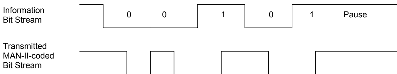
Figure 19: Manchester-II-Modulation principle
