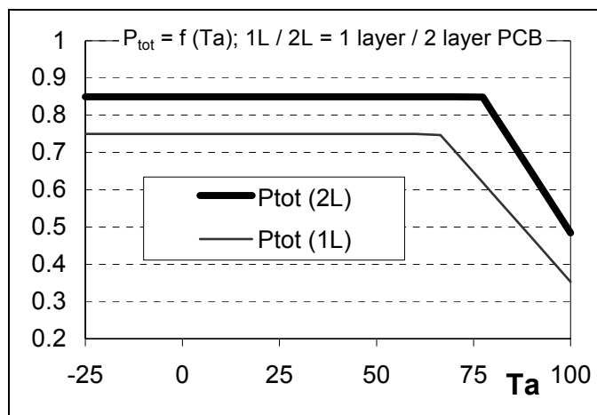
Figure 1: P_{tot} = f(\theta_a)
