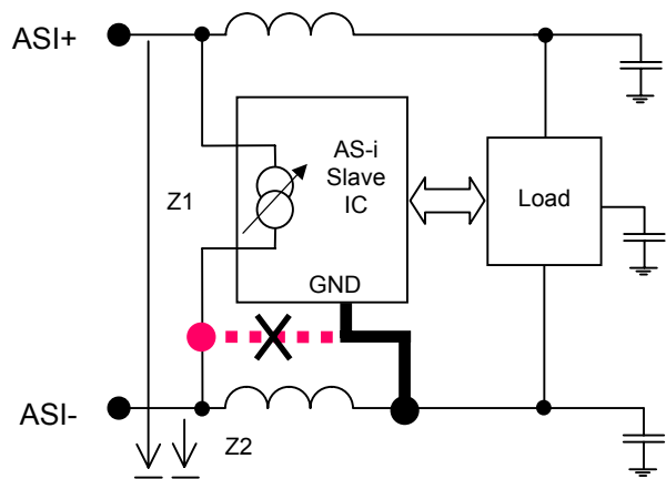
Figure 4: Newly supported application of AS-i IC with two external coils
