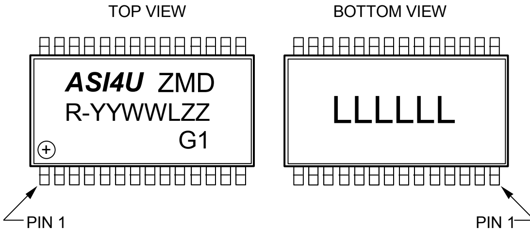
Figure 25: Package Marking
