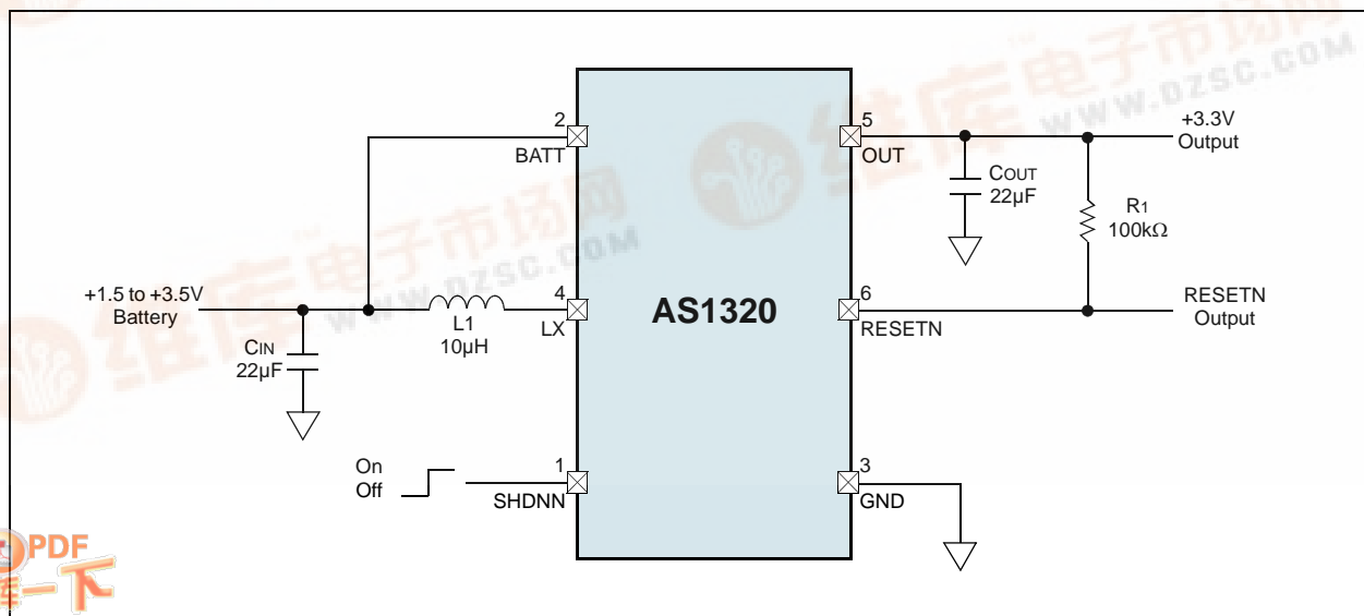
Figure 1. Application Diagram
