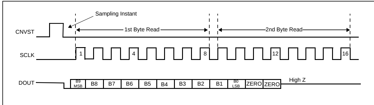
Figure 24. SPI/Microwire Interface Timing Diagram (CPOL = CPHA = 0)
