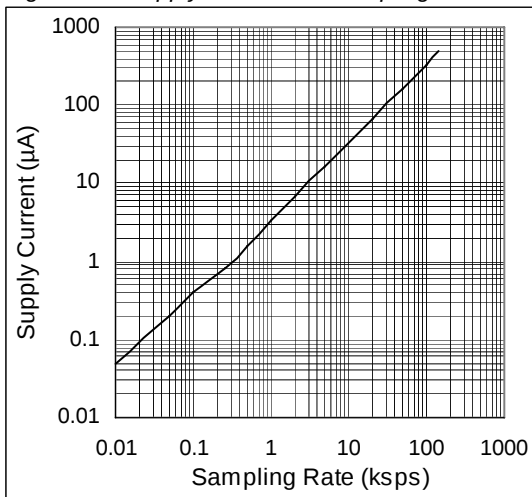
Figure 10. Supply Current vs. Sampling Rate
