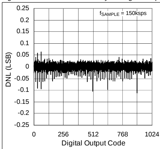
Figure 6. Differential Nonlinearity vs. Digital Output Code
