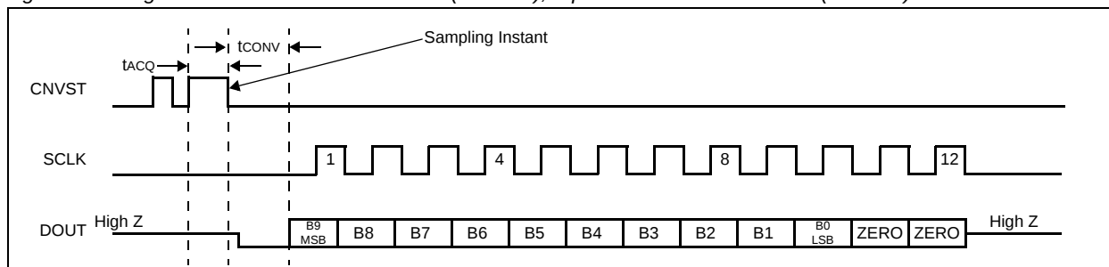
Figure 19. Single Conversion – AIN2 vs. GND (AS1529), Bipolar Mode AIN+ vs. AIN- (AS1528)
