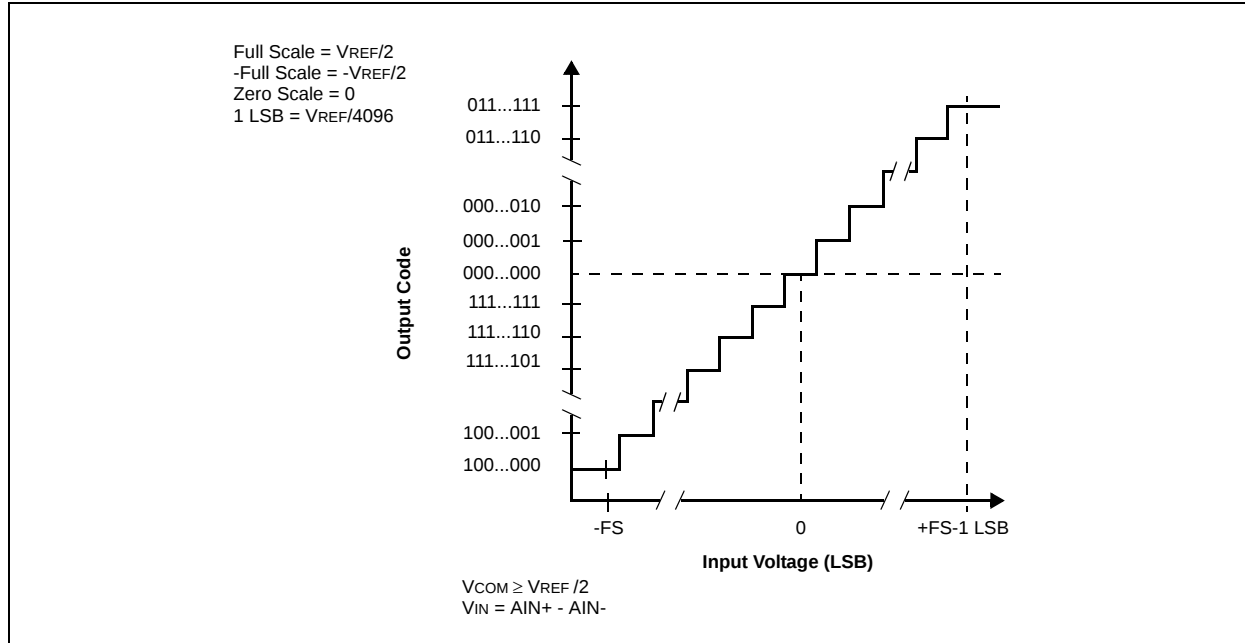
Figure 21. AS1528 Bipolar Transfer Function
