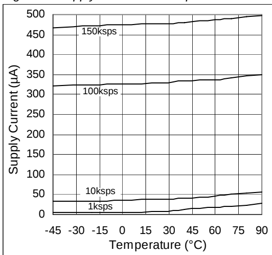
Figure 8. Supply Current vs. Temperature
