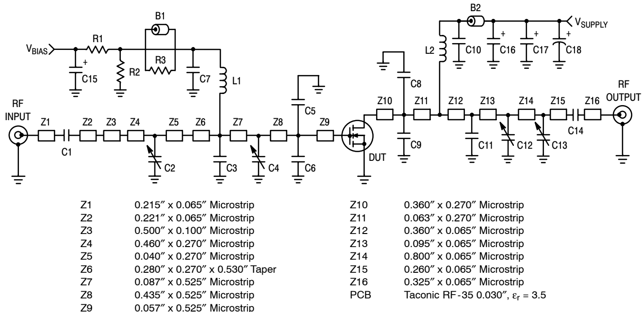
Figure 1. MRFE6S9045NR1 Test Circuit Schematic
