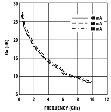
Figure 11. Ga vs. Frequency vs. I_{ds} , V_{ds} = 3V^{[1]} .
