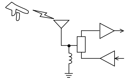
Figure 23. In-circuit ESD Protection.
