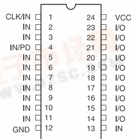
DIP/SOIC
