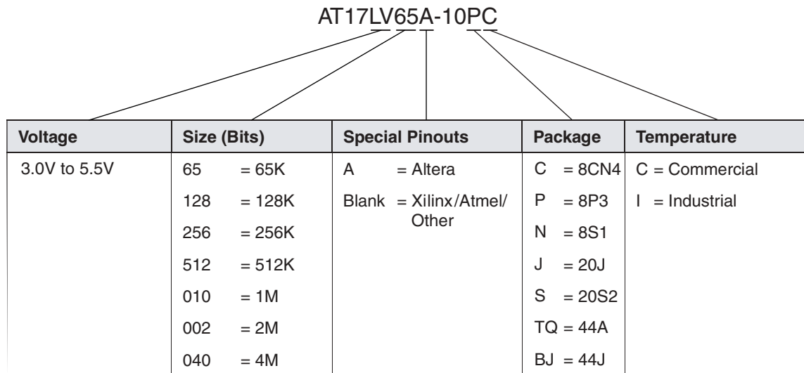
Figure 1. Ordering Code
