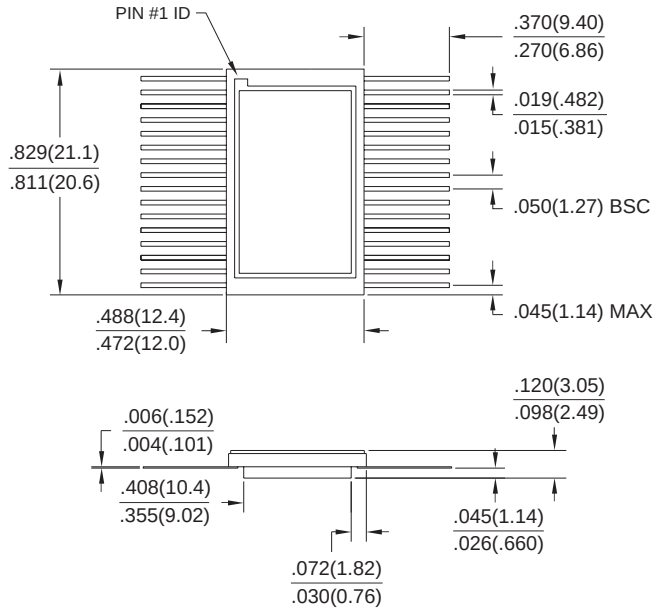
32F, 32-Lead, Non-Windowed, Ceramic Bottom-Brazed Flat Package (Flatpack) Dimension in Inches and (Millimeters) JEDEC OUTLINE MO-115
