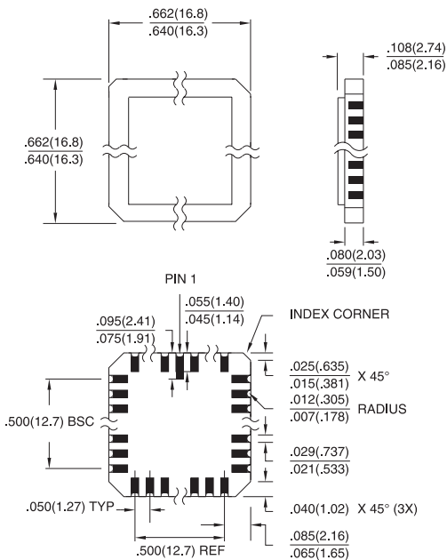
44L, 44-Pad, Non-Windowed, Ceramic Leadless Chip Carrier (LCC) Dimensions in Inches and (Millimeters)* MIL-STD-1835 C-5
