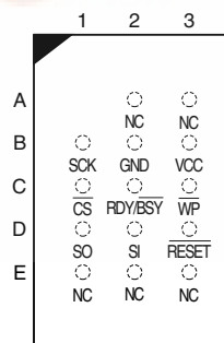
CBGA Top View Through Package
