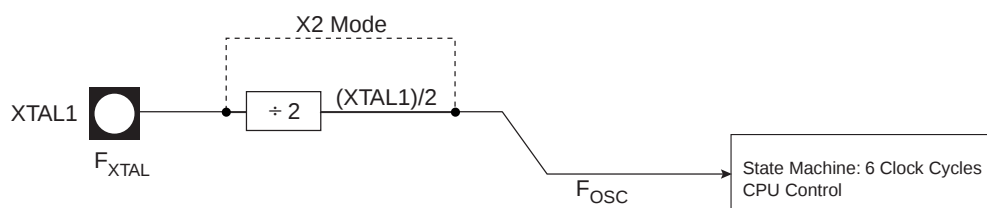
Figure 3. Clock Generation Block Diagram
