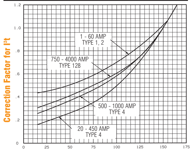
Clearing I 2 t vs Working Voltage
