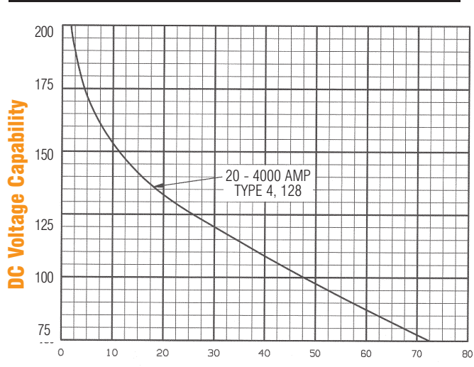
DC Voltage vs Time Constant (L/R)
