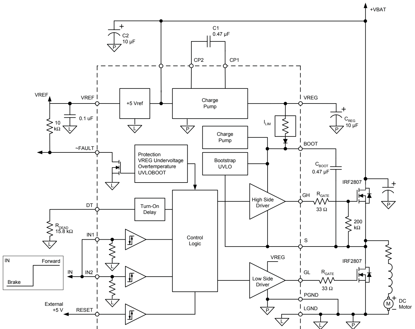
Diagram A. Dependent drivers. Unidirectional motor control with braking and dead time. T_{\text{DEAD}} = 1 \mu\text{s} ; Q_{\text{TOTAL}} = 160 \text{ nC} .
