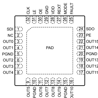
Pin-out Diagram
