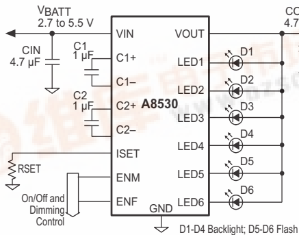
Figure 1. 4×30 mA backlight with 2×100 mA flash
