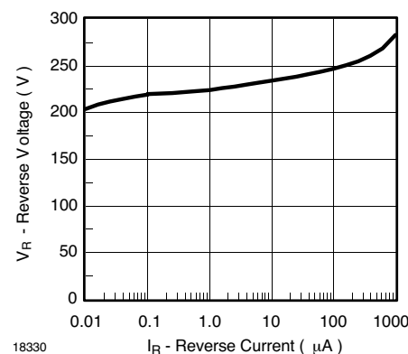
Fig. 4 Reverse Voltage vs. Reverse Current
