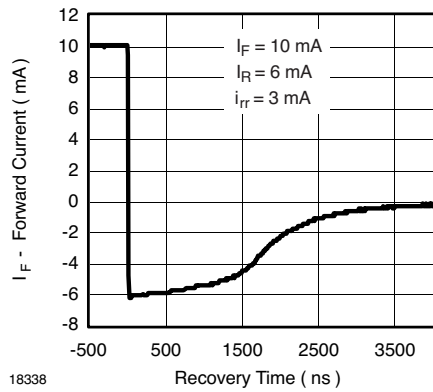
Fig. 5 Typical Charge Recovery Curve
