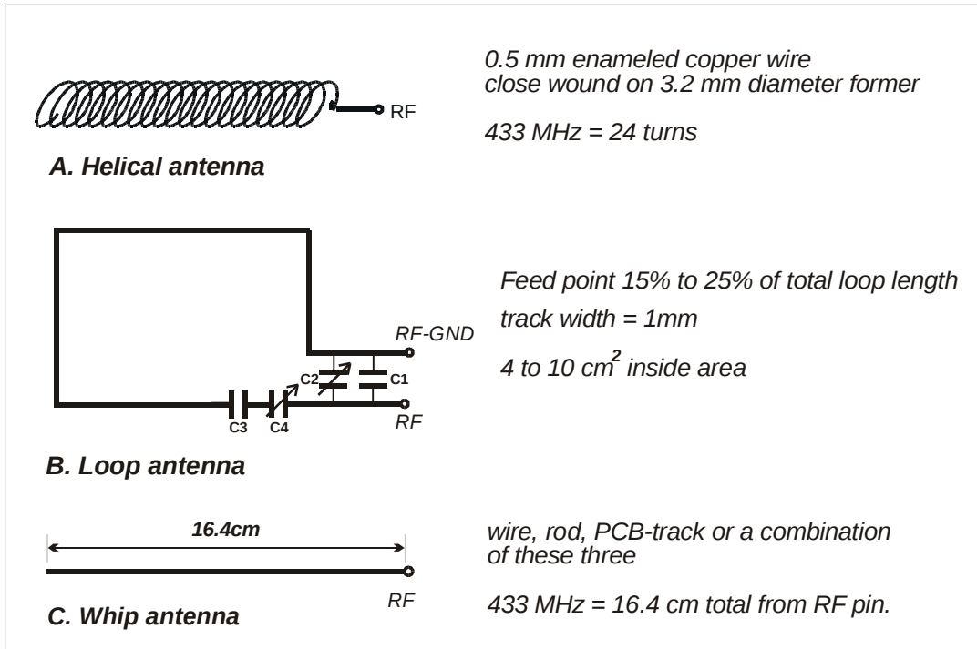
Fig. 5: Antenna configurations
