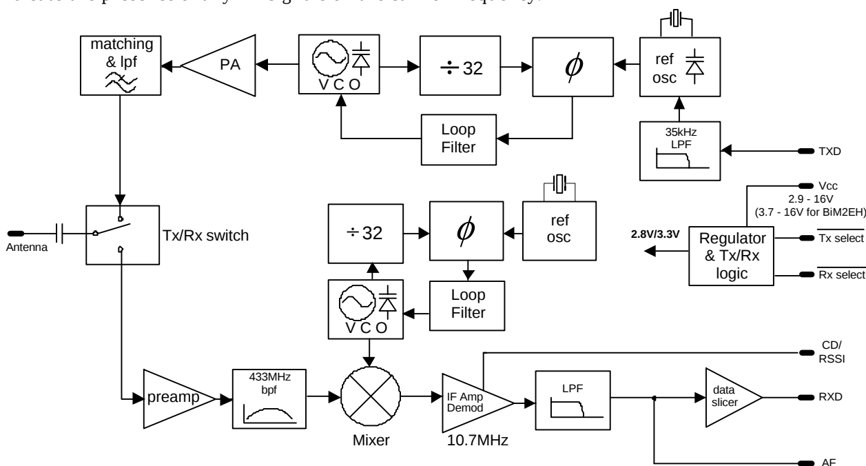
Fig. 2: Block diagram
