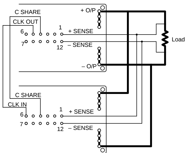
Parallel Connections
