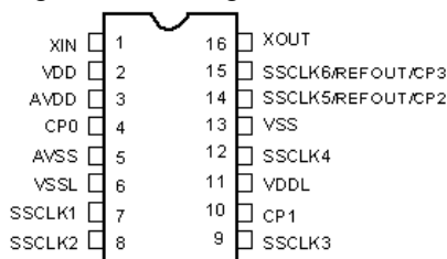
Figure 1. Pin Diagram
