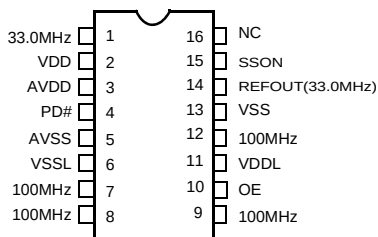
Figure 2. Pin Diagram
