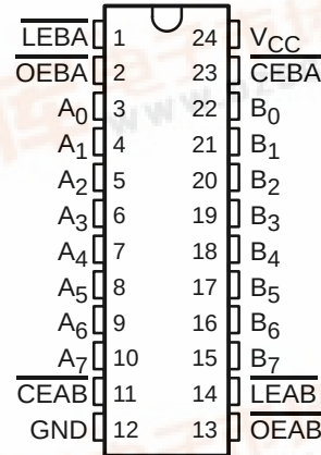
CY54FCT543T . . . D PACKAGE CY74FCT543T . . . Q OR SO PACKAGE (TOP VIEW)
