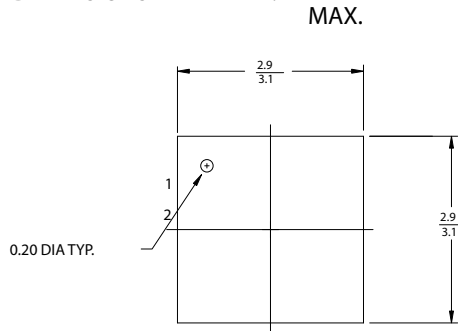
Figure 4. 16L Chip On Lead 3 X 3 mm Package Outline (SAWN) - 001-09116 - (Pb-Free)
