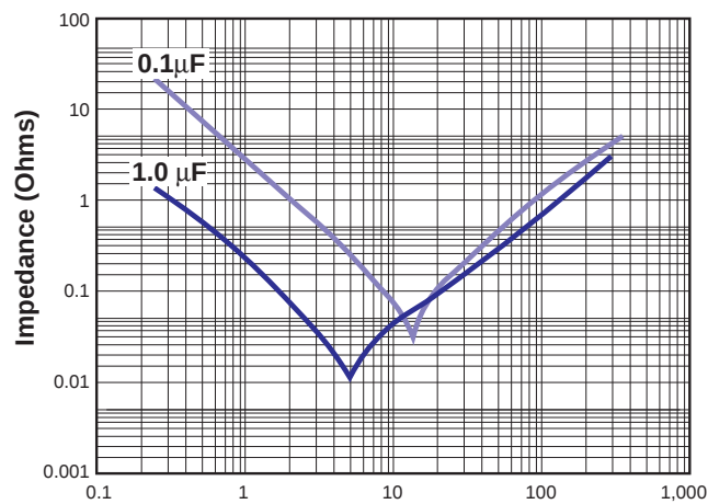
Figure 12. Impedance vs Frequency for Z5U Dielectric
