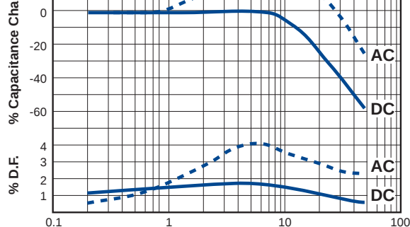
Figure 7. AC or DC Volts Applied Typical Effects of 1000 Hz AC and DC Voltage Level on Capacitance and Dissipation Factor - Z5U
