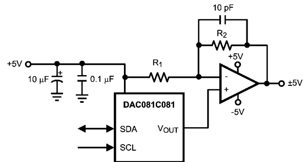
FIGURE 14. Bipolar Operation
