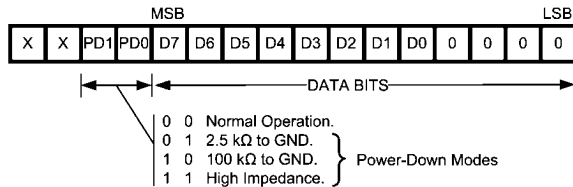
FIGURE 8. DAC Register Contents
