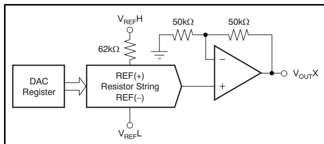
Figure 92. DAC8565 Architecture
