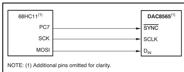
Figure 103. DAC8565 to 68HC11 Interface
