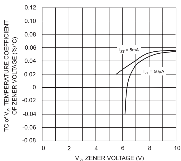
Fig. 15 Typical Temperature Coefficient of Zener Voltage vs. Zener Voltage, DDZX6V2B-DDZX10C
