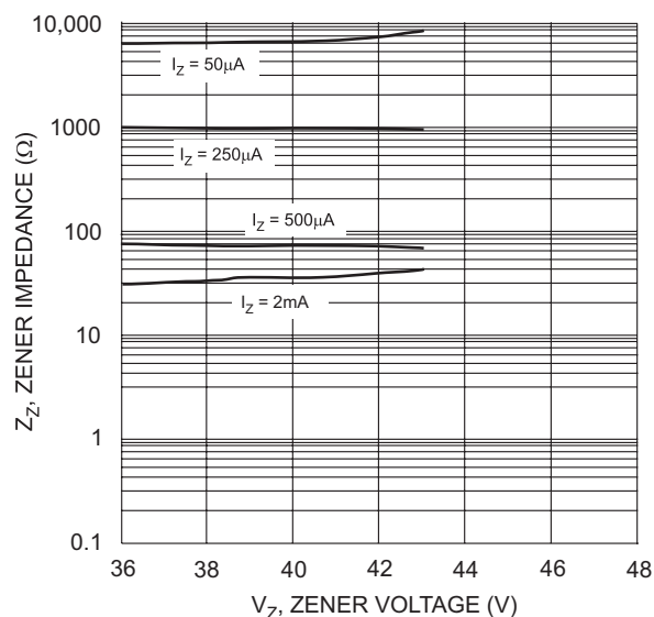
Fig. 14 Typical Zener Impedance Characteristics, DDZX36 - DDZX43
