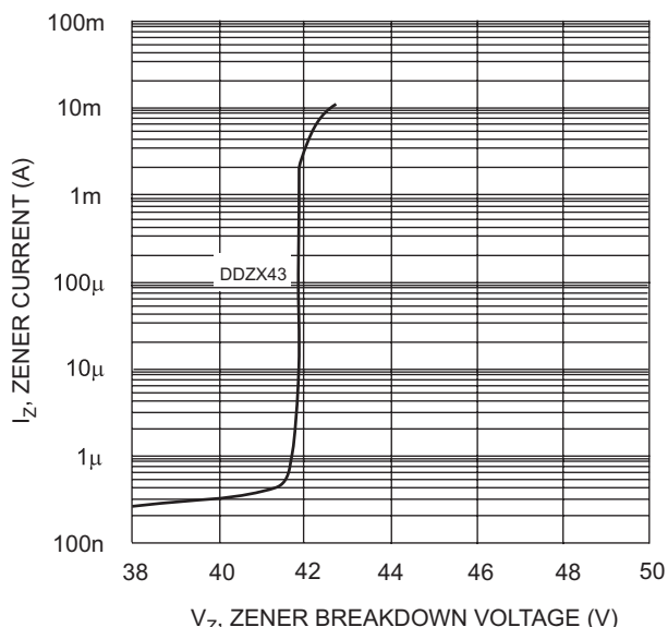
Fig. 9 Typical Reverse Characteristics, DDZX43
