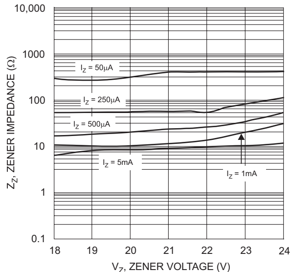
Fig. 12 Typical Zener Impedance Characteristics, DDZX18C - DDZX24C
