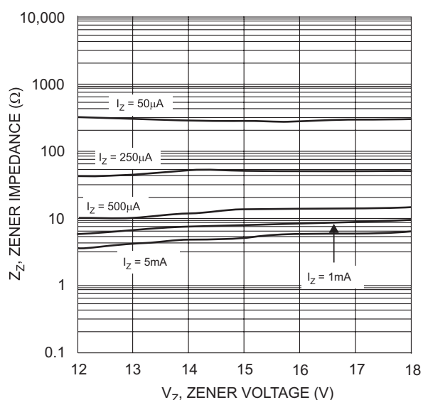
Fig. 11 Typical Zener Impedance Characteristics, DDZX12C - DDZX18C
