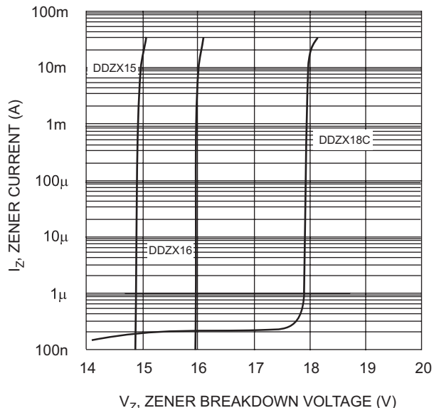
Fig. 6 Typical Reverse Characteristics, DDZX15 - DDZX18C
