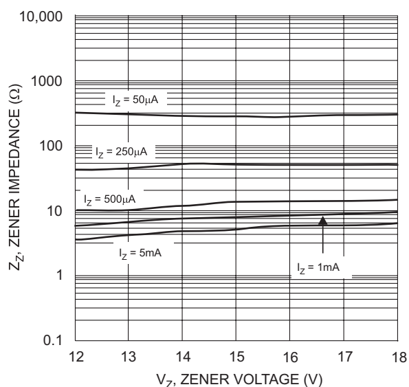
Fig. 11 Typical Zener Impedance Characteristics, DDZX12CTS - DDZX18CTS
