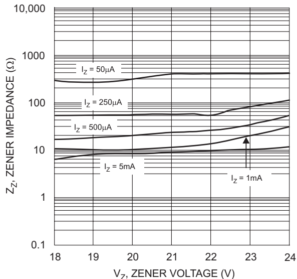
Fig. 12 Typical Zener Impedance Characteristics, DDZX18CTS - DDZX24CTS
