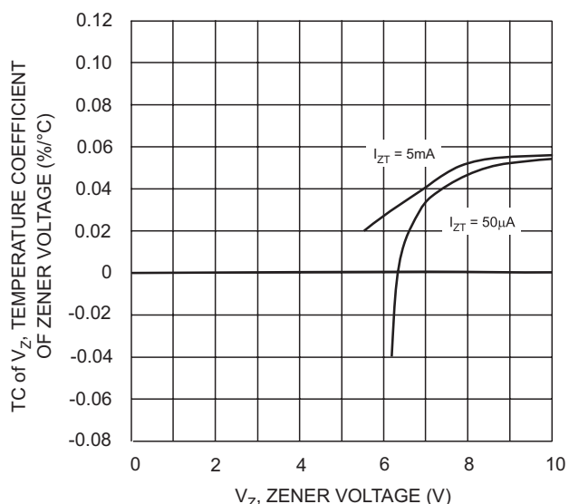
Fig. 15 Typical Temperature Coefficient of Zener Voltage vs. Zener Voltage, DDZX6V62TS-DDZX10CTS
