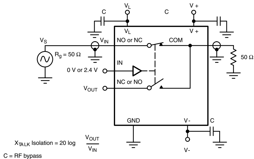
Figure 6. Crosstalk (DG419L)
