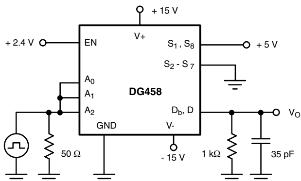
Figure 4. Break-Before-Make Time
