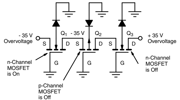
(a) Overvoltage with Multiplexer Power Off
