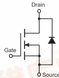
EQUIVALENT CIRCUIT
