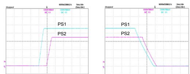
Figure 40: Sequential Start-up
