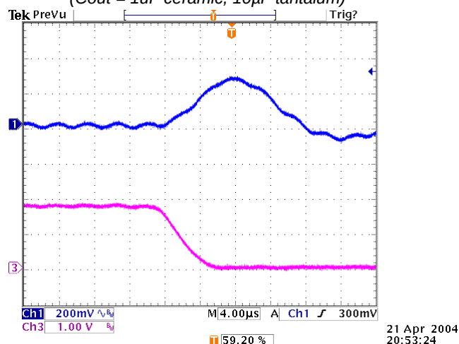
Figure 21: Typical transient response to step load change at 2.5\text{A}/\mu\text{s} from 100% to 50% of I_o , max at 5V_{in} , 1.8V_{out} ( C_{out} = 1\mu\text{F} ceramic, 10\mu\text{F} tantalum)
