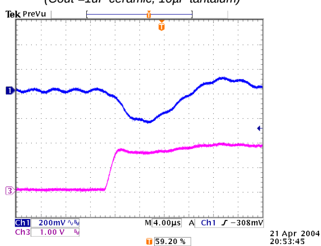
Figure 22: Typical transient response to step load change at 2.5\text{A}/\mu\text{s} from 50% to 100% of I_o , max at 5V_{in} , 1.8V_{out} ( C_{out} = 1\mu\text{F} ceramic, 10\mu\text{F} tantalum)
