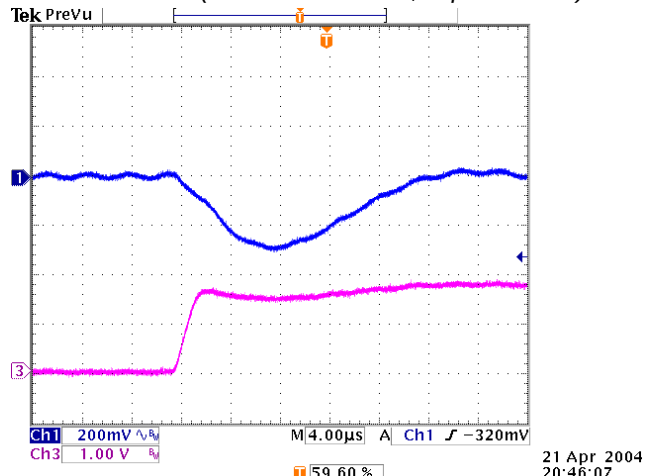
Figure 26: Typical transient response to step load change at 2.5\text{A}/\mu\text{s} from 50% to 100% of I_o , max at 3.3\text{V}_{in} , 1.8\text{V}_{out} ( C_{out} = 1\mu\text{F} ceramic, 10\mu\text{F} tantalum)
