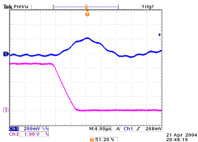
Figure 19: Typical transient response to step load change at 2.5\text{A}/\mu\text{s} from 100% to 50% of I_o , max at 5V_{in} , 3.3V_{out} ( C_{out} = 1\mu\text{F} ceramic, 10\mu\text{F} tantalum)
