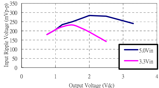
Figure 32: Input voltage ripple for various output models, I_O = 10 \text{ A} ( C_{IN} = 2 \times 100 \text{ µF} tantalum // 47 \text{ µF} ceramic)
