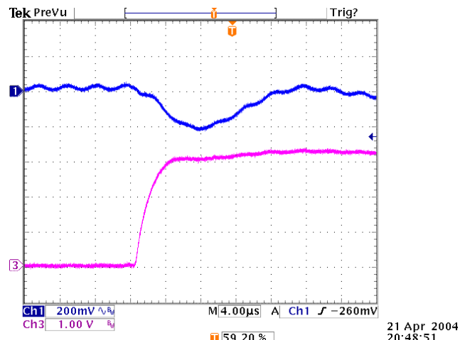
Figure 20: Typical transient response to step load change at 2.5\text{A}/\mu\text{s} from 50% to 100% of I_o , max at 5V_{in} , 3.3V_{out} ( C_{out} = 1\mu\text{F} ceramic, 10\mu\text{F} tantalum)
