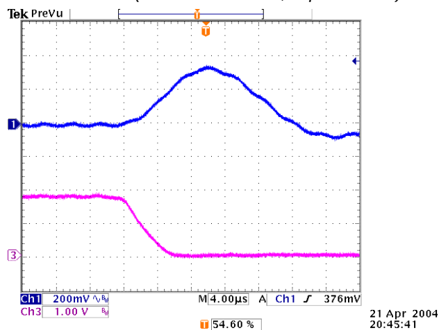
Figure 25: Typical transient response to step load change at 2.5\text{A}/\mu\text{s} from 100% to 50% of I_o , max at 3.3\text{V}_{in} , 1.8\text{V}_{out} ( C_{out} = 1\mu\text{F} ceramic, 10\mu\text{F} tantalum)
