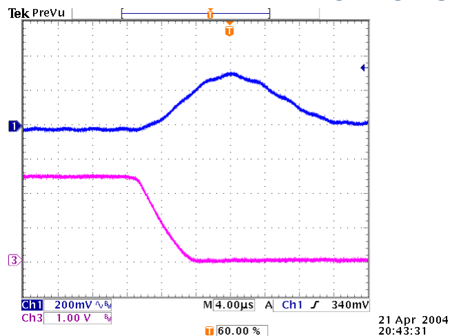
Figure 23: Typical transient response to step load change at 2.5\text{A}/\mu\text{s} from 100% to 50% of I_o , max at 3.3\text{V}_{in} , 2.5\text{V}_{out} ( C_{out} = 1\mu\text{F} ceramic, 10\mu\text{F} tantalum)
