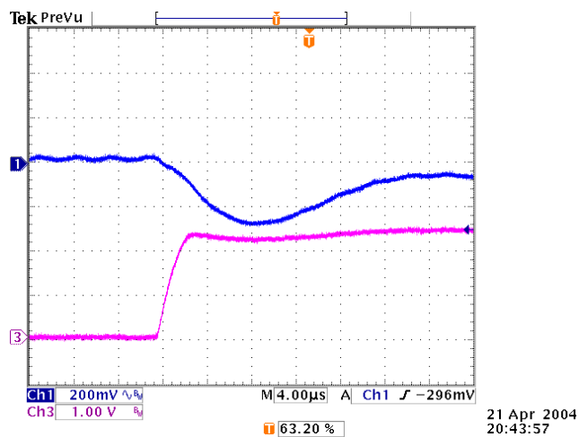
Figure 24: Typical transient response to step load change at 2.5\text{A}/\mu\text{s} from 50% to 100% of I_o , max at 3.3\text{V}_{in} , 2.5\text{V}_{out} ( C_{out} = 1\mu\text{F} ceramic, 10\mu\text{F} tantalum)
