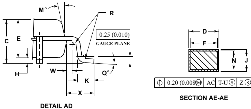
Figure 5-2 100-pin LQFP Mechanical Information
