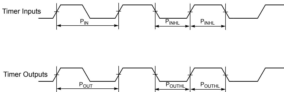
Figure 4-25 Timer Timing
