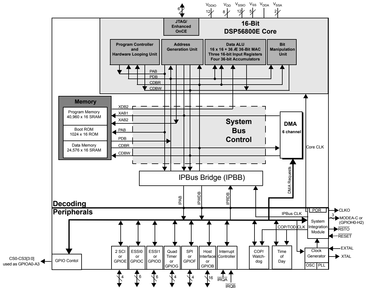
56857 Block Diagram
