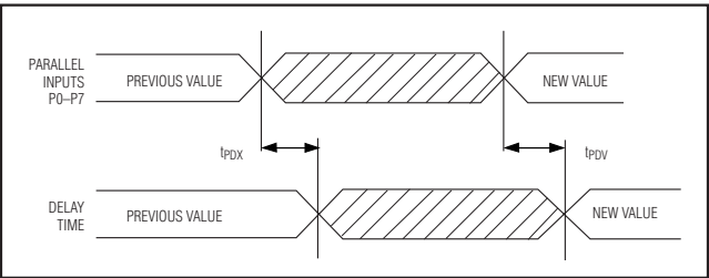
Figure 3. Nonlatched Parallel Timing Diagram
