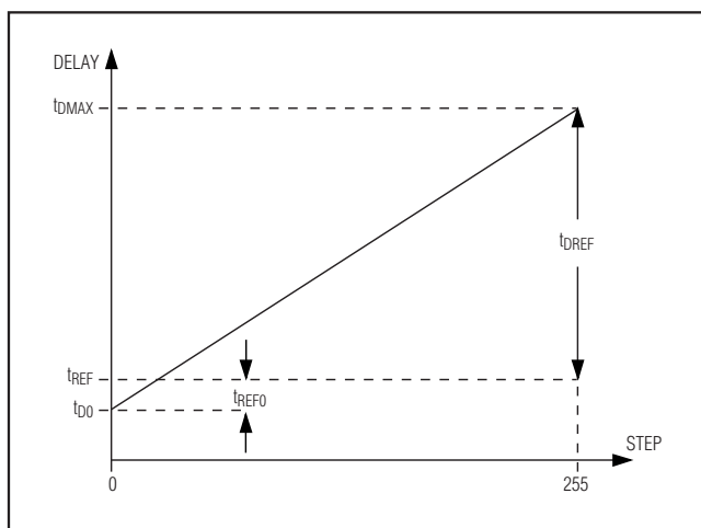
Figure 8. Delay Parameters
