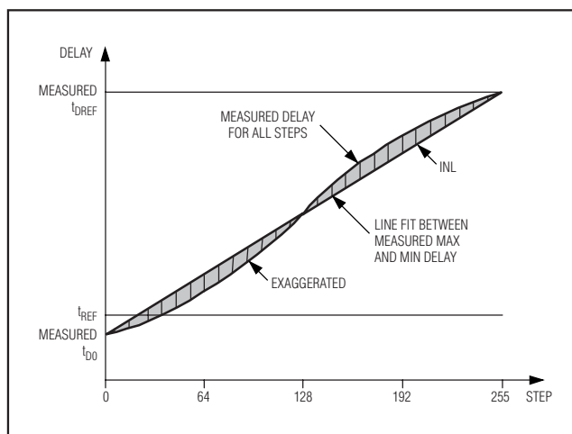
Figure 9. Integral Nonlinearity
