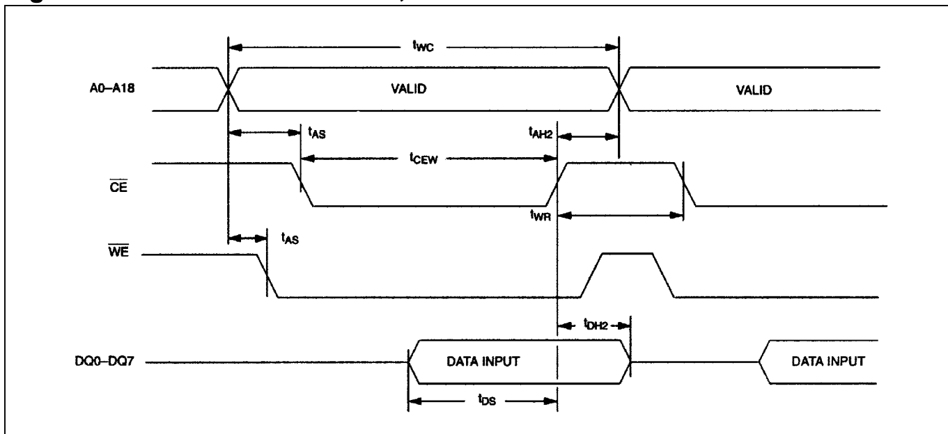
Figure 7. WRITE CYCLE TIMING, CHIP-ENABLE CONTROLLED
