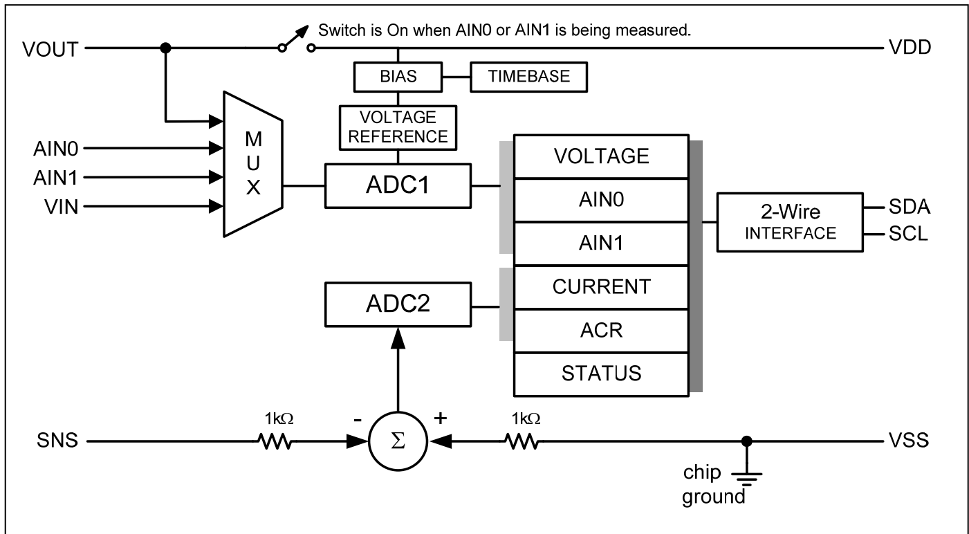
Figure 2. Block Diagram
