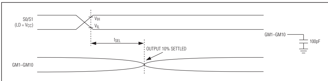
Figure 3. Input Pin to Output Change Timing Diagram
