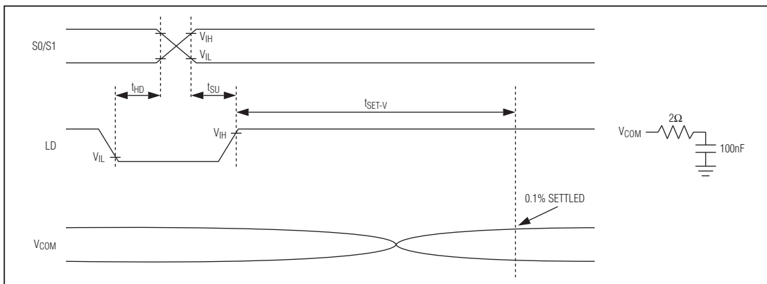
Figure 1. V COM Settling Timing Diagram
