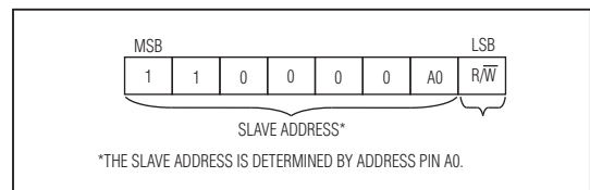
Figure 5. DS3510 Slave Address Byte
