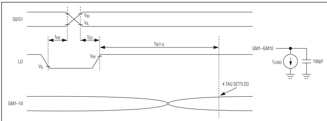
Figure 2. GM1-10 Settling Timing Diagram
