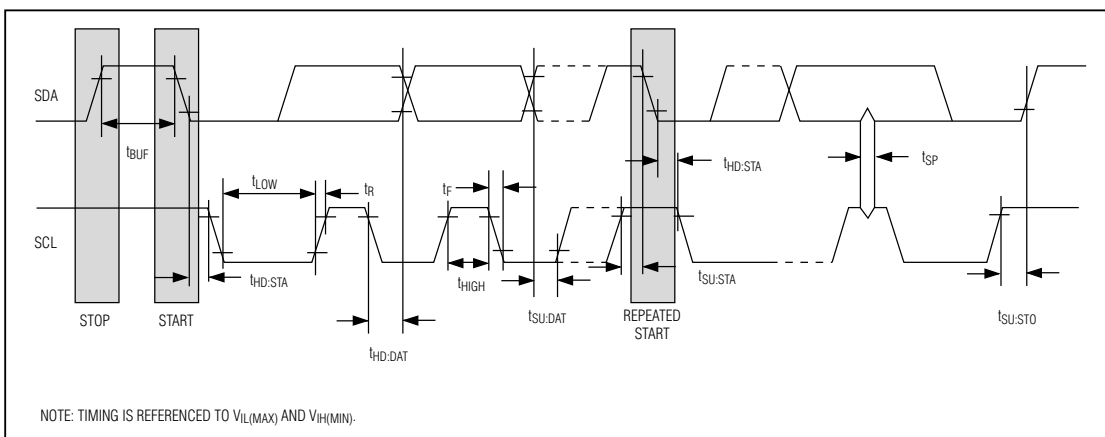
Figure 4. I 2 C Timing Diagram
