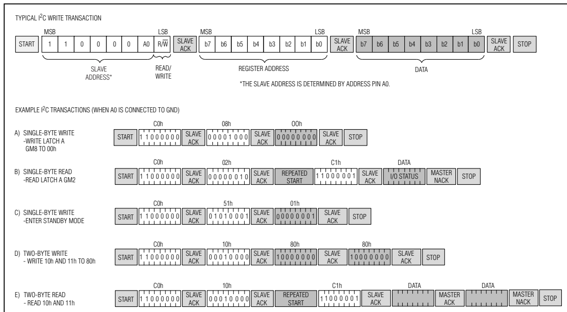
Figure 6. I 2 C Communication Examples
