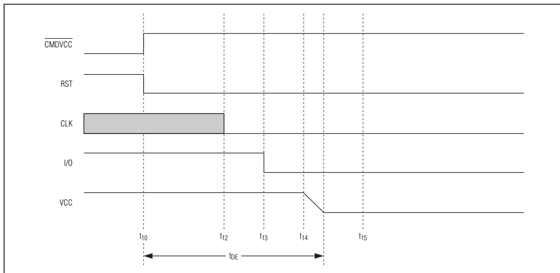
Figure 5. Deactivation Sequence
