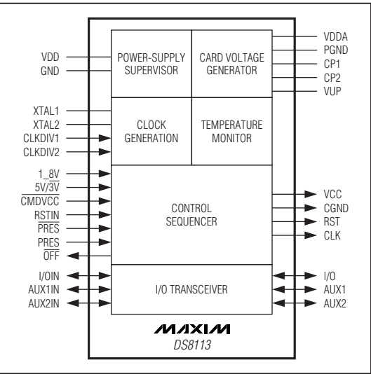
Figure 1. Functional Diagram
