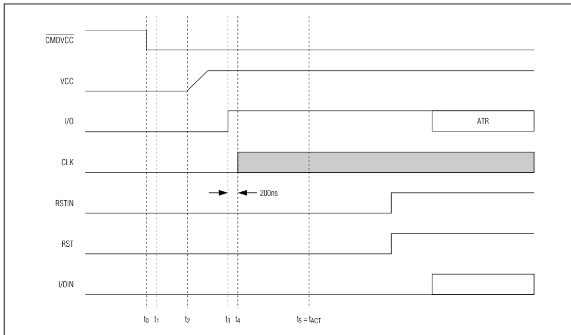
Figure 4. Activation Sequence at t_3
