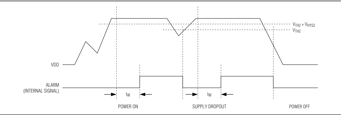
Figure 2. Voltage Supervisor Behavior
