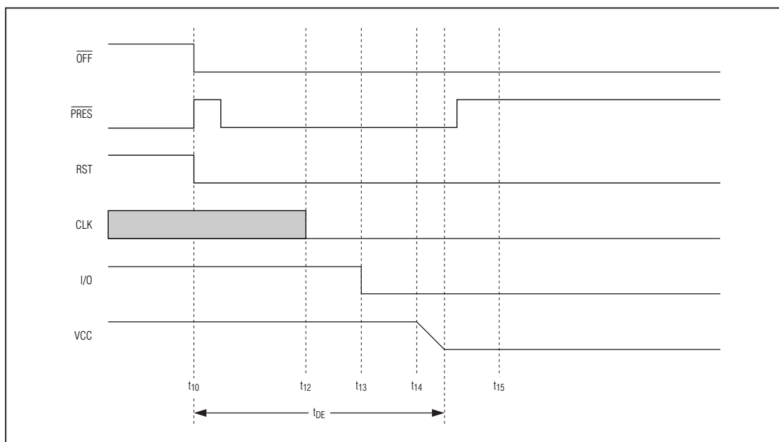
Figure 7. Emergency Deactivation Sequence (Card Extraction)
