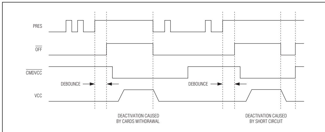
Figure 6. Behavior of PRES, \overline{\text{OFF}} , \overline{\text{CMDVCC}} , and VCC
