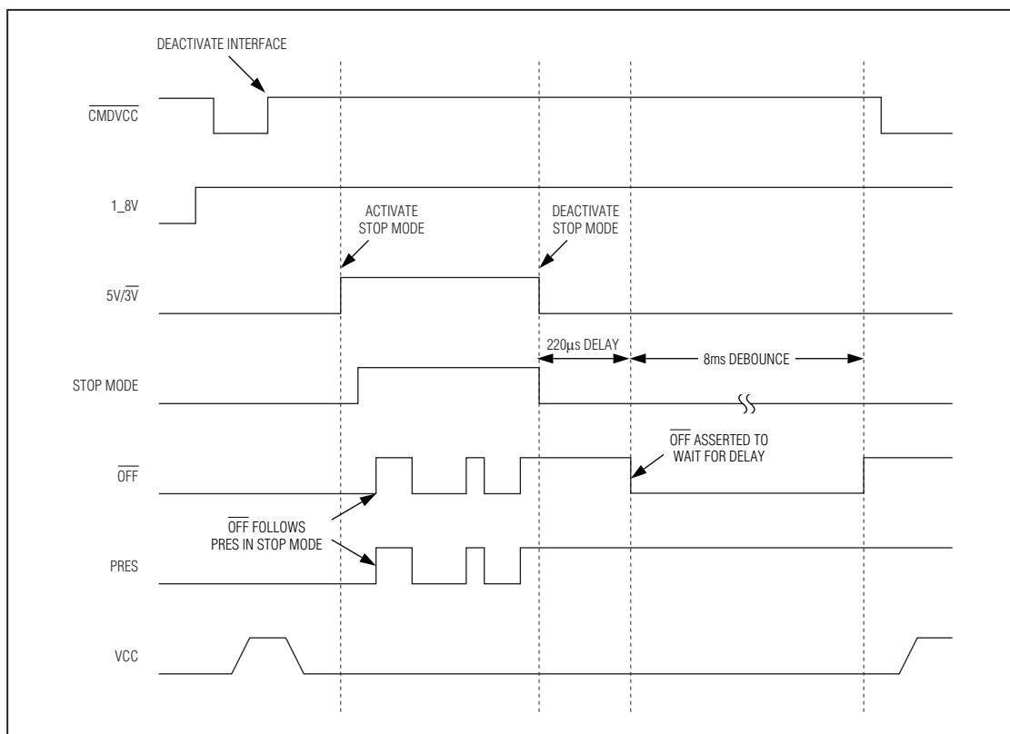
Figure 8. Stop-Mode Sequence
