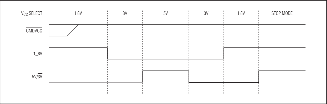
Figure 9. Smart Card Power Select
