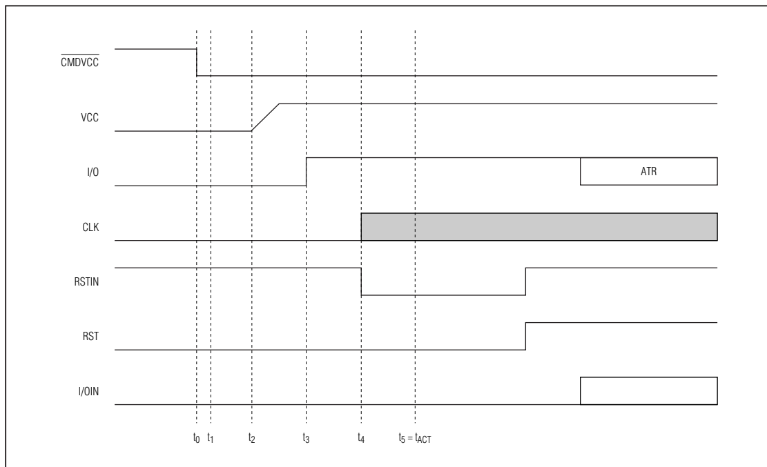
Figure 3. Activation Sequence Using RSTIN and \overline{\text{CMDVCC}}
