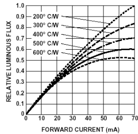
Figure 4. HPWT-xx00 Relative Luminous Flux vs. Forward Current.
