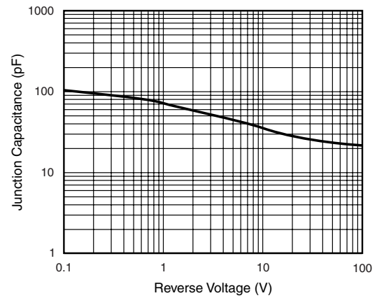
Figure 5. Typical Capacitance
