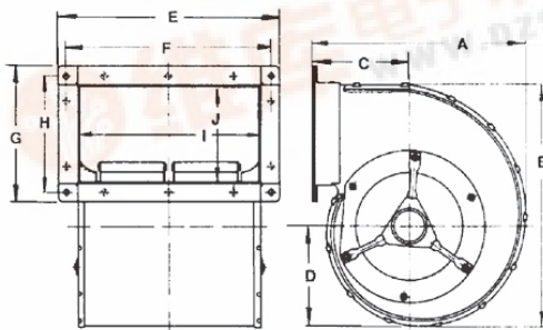
DIMENSIONS - Inches (mm)
