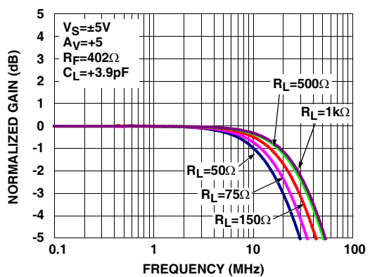
FIGURE 10. GAIN vs FREQUENCY FOR VARIOUS R_{LOAD} ( A_V = +5 )
