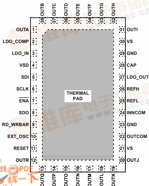
EL5625 (38-PIN QFN) TOP VIEW
